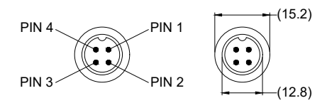
4 PIN MALE MATING FACE
